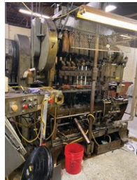
WATERBURY FARRELL 2010 EYELET TRANSFER PRESS
